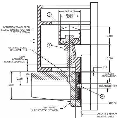
AMPS system with five rings of DualPac 2212 packing.
